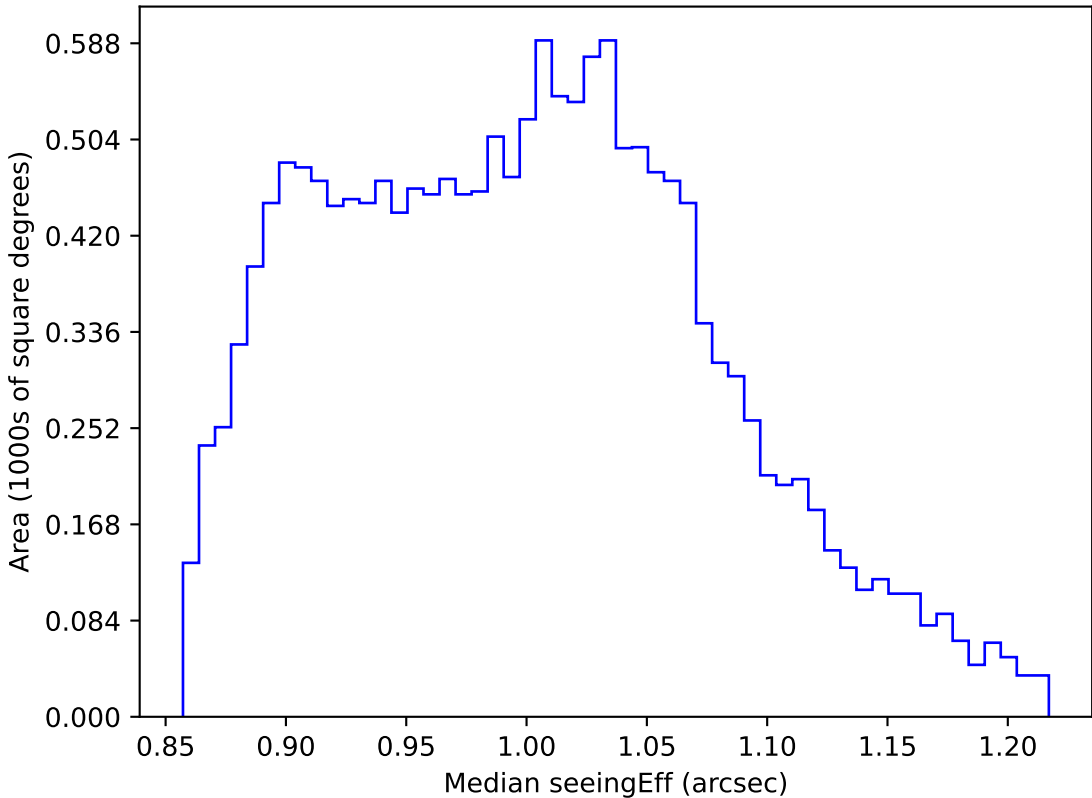
too_elab_r256_d3_ugrizy_v3.4_10yrs WFD i band: Median seeingEff
