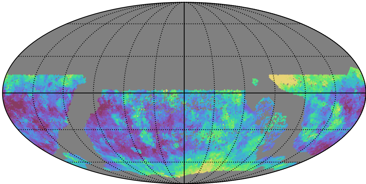
too_elab_r256_d3_ugrizy_v3.4_10yrs WFD g band: Median seeingEff
