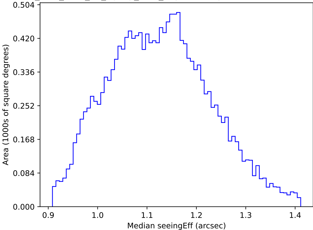
too_elab_r256_d3_ugrizy_v3.4_10yrs WFD g band: Median seeingEff
