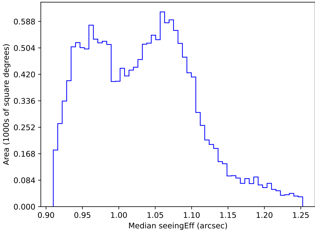
too_elab_r256_d3_ugrizy_v3.4_10yrs WFD all bands: Median seeingEff
