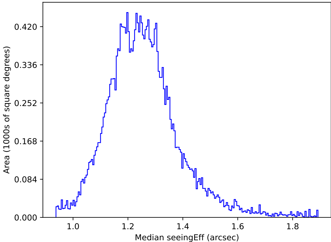
too_elab_r256_d3_ugrizy_v3.4_10yrs All sky u band: Median seeingEff
