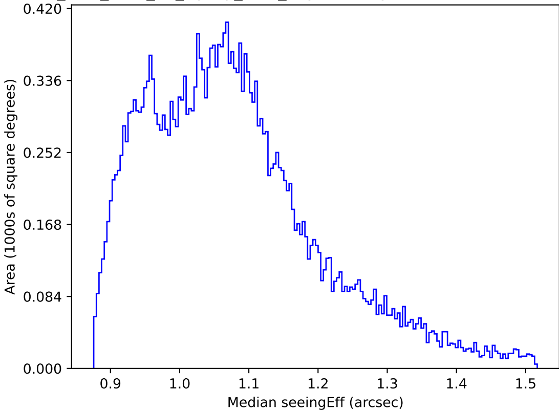
too_elab_r256_d3_ugrizy_v3.4_10yrs All sky r band: Median seeingEff
