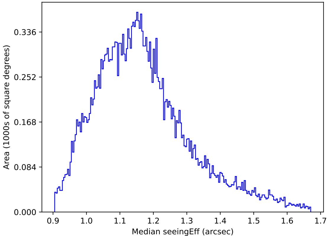
too_elab_r256_d3_ugrizy_v3.4_10yrs All sky g band: Median seeingEff
