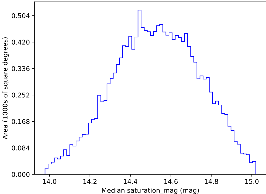
too_elab_r256_d3_ugrizy_v3.4_10yrs WFD g band: Median saturation_mag
