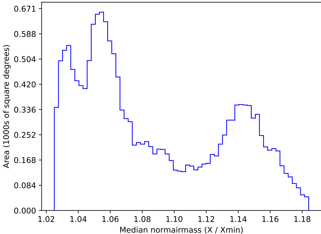
too_elab_r256_d3_ugrizy_v3.4_10yrs WFD all bands: Median normairmass
