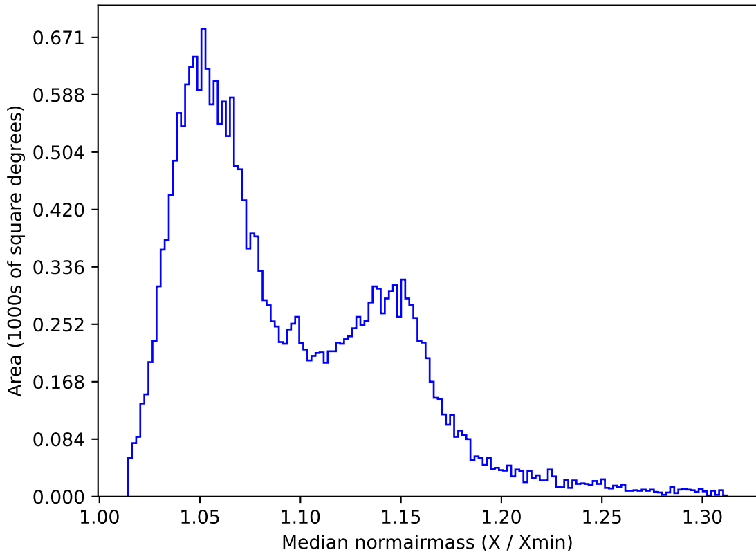
too_elab_r256_d3_ugrizy_v3.4_10yrs All sky y band: Median normairmass
