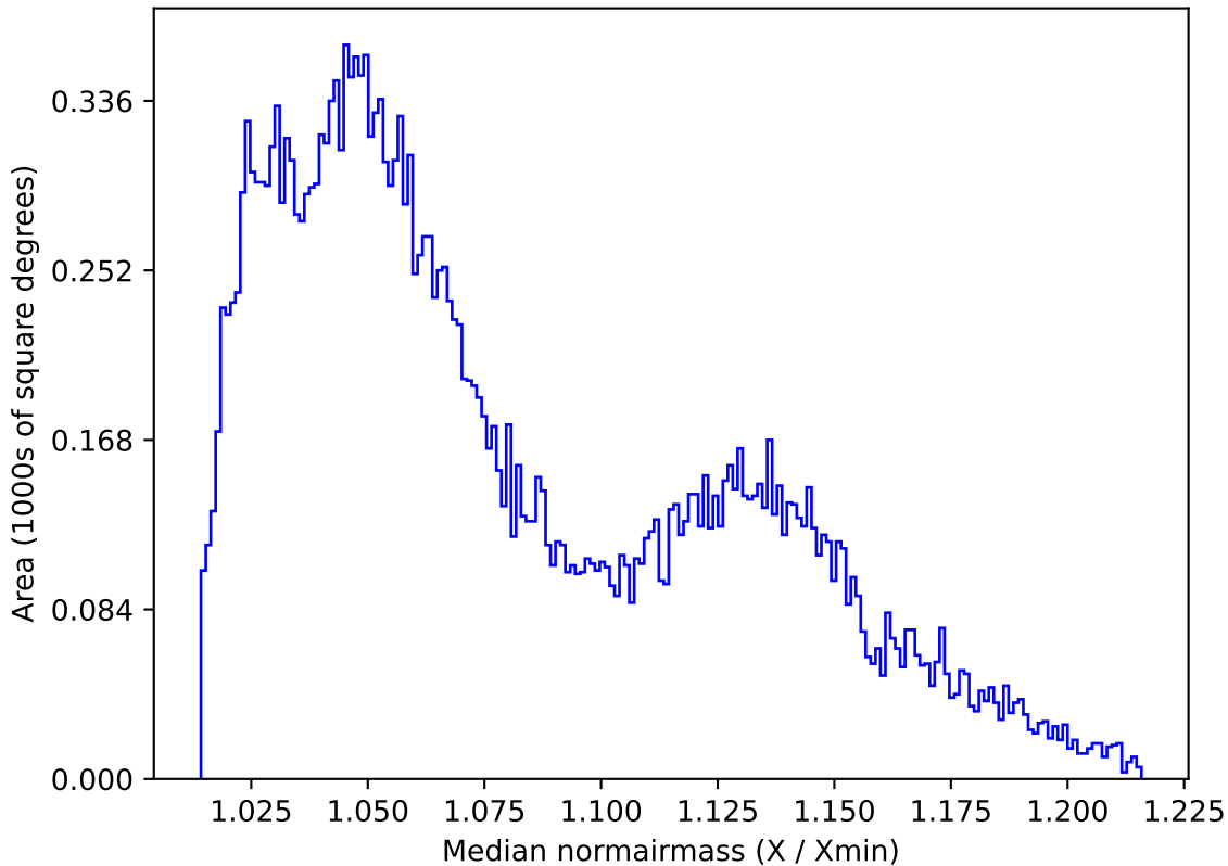
too_elab_r256_d3_ugrizy_v3.4_10yrs All sky r band: Median normairmass
