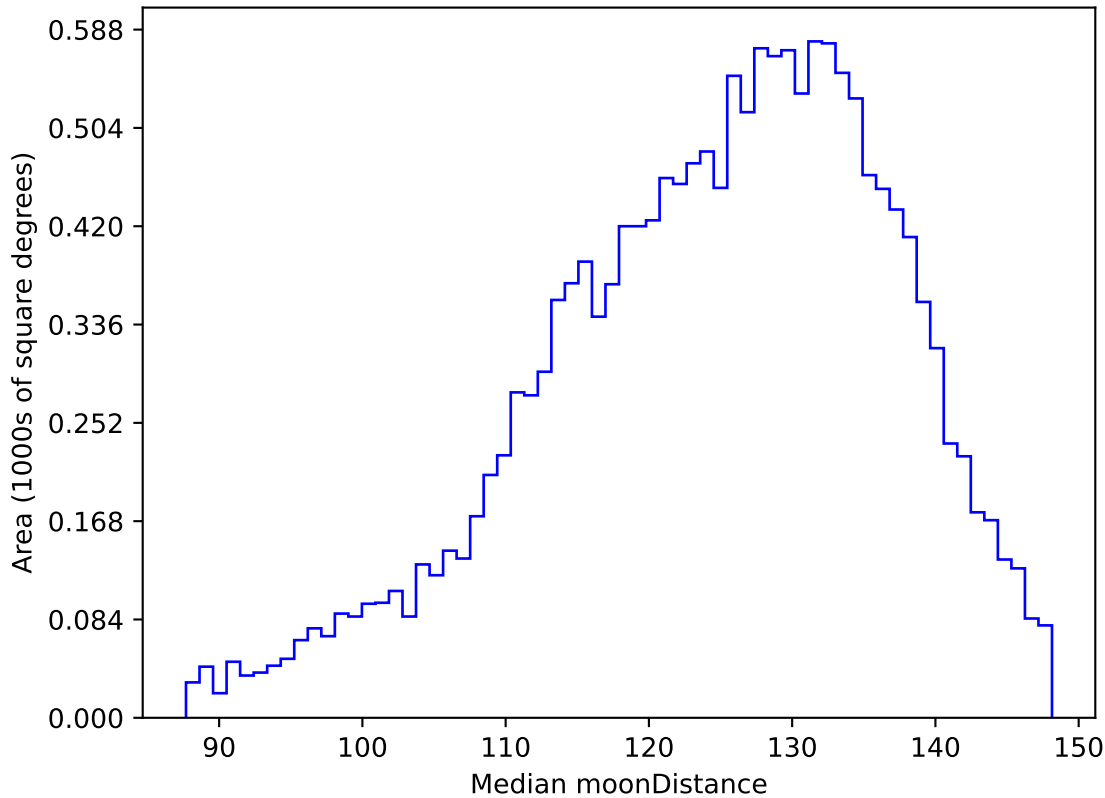
too_elab_r256_d3_ugrizy_v3.4_10yrs WFD u band: Median moonDistance
