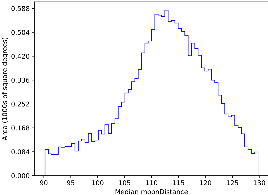
too_elab_r256_d3_ugrizy_v3.4_10yrs WFD r band: Median moonDistance
