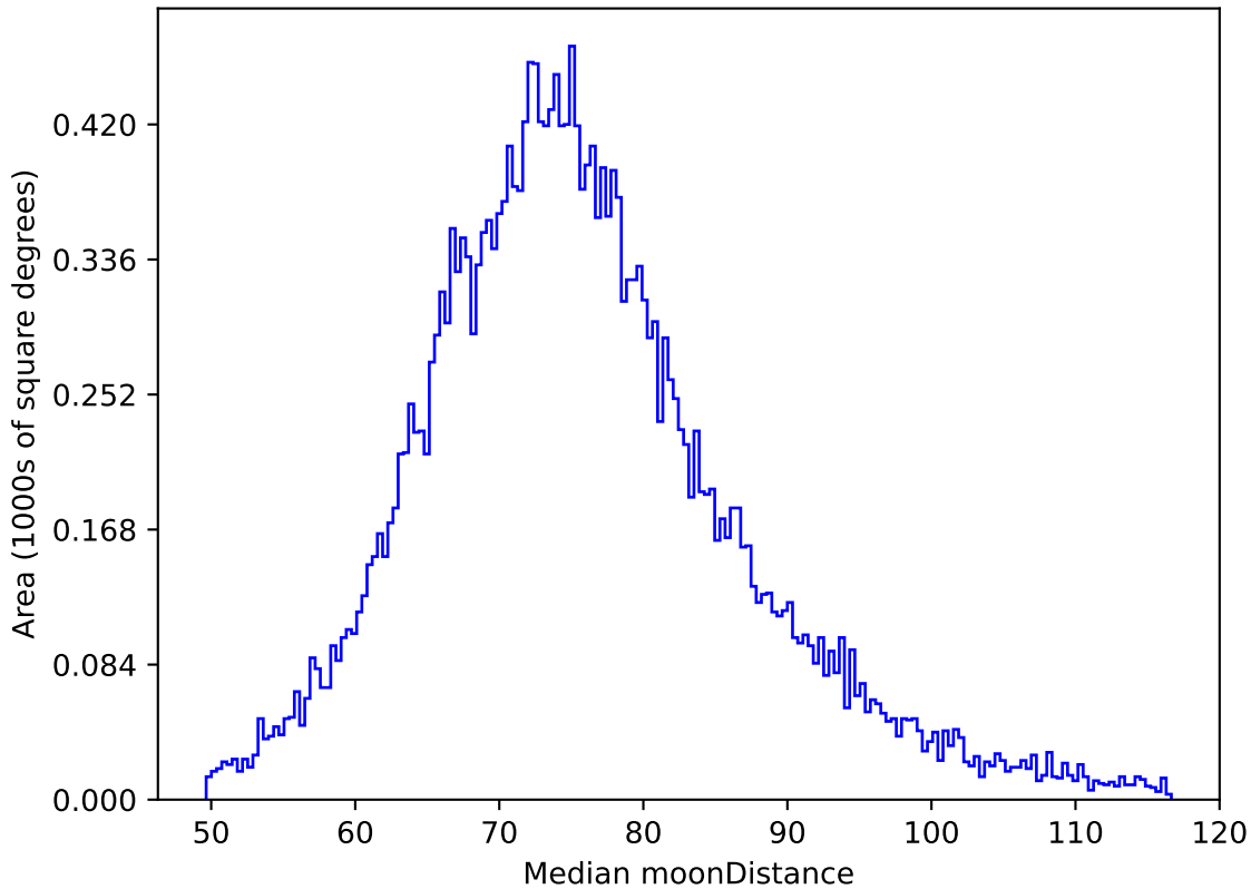
too_elab_r256_d3_ugrizy_v3.4_10yrs All sky z band: Median moonDistance
