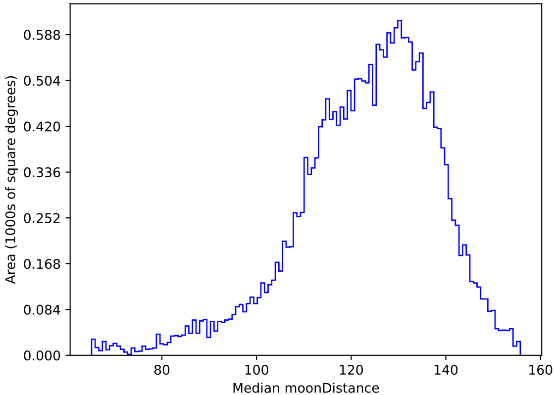
too_elab_r256_d3_ugrizy_v3.4_10yrs All sky u band: Median moonDistance
