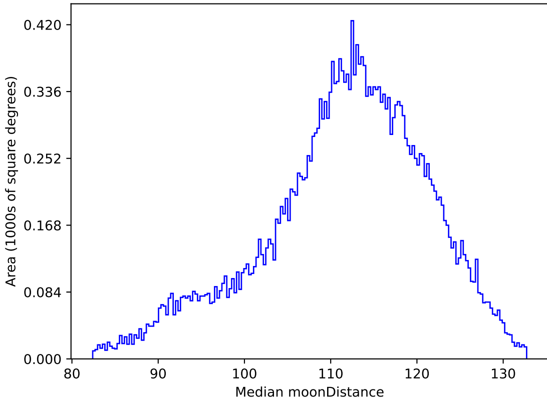
too_elab_r256_d3_ugrizy_v3.4_10yrs All sky r band: Median moonDistance
