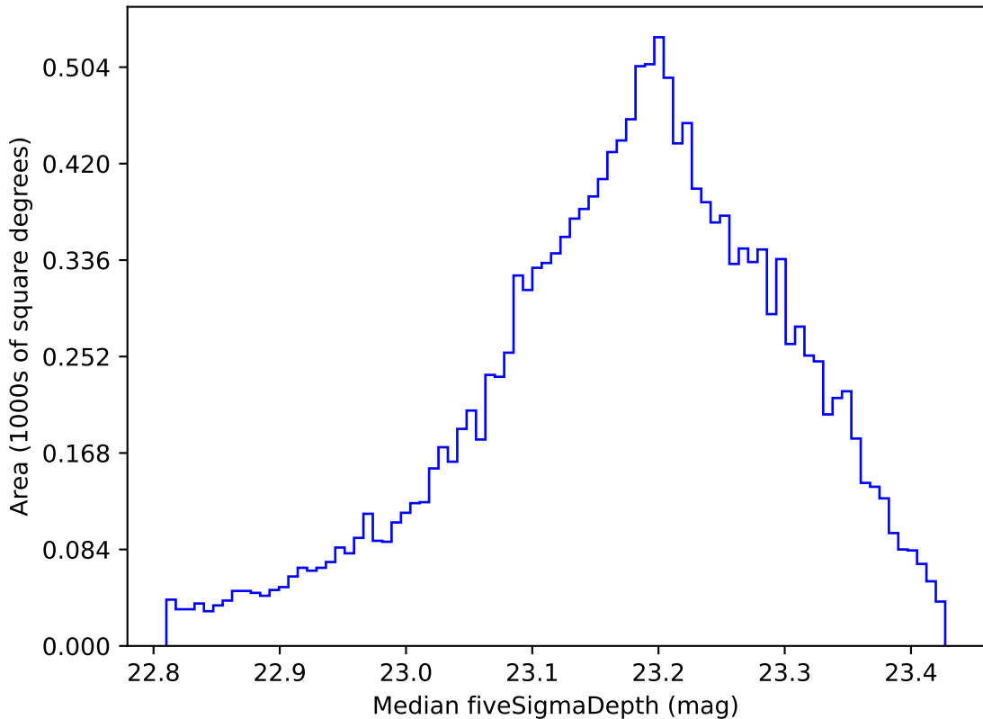
too_elab_r256_d3_ugrizy_v3.4_10yrs WFD u band: Median fiveSigmaDepth
