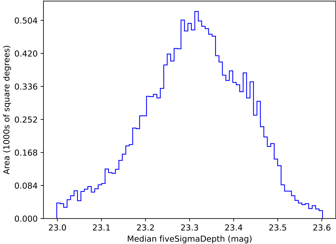
too_elab_r256_d3_ugrizy_v3.4_10yrs WFD all bands: Median fiveSigmaDepth
