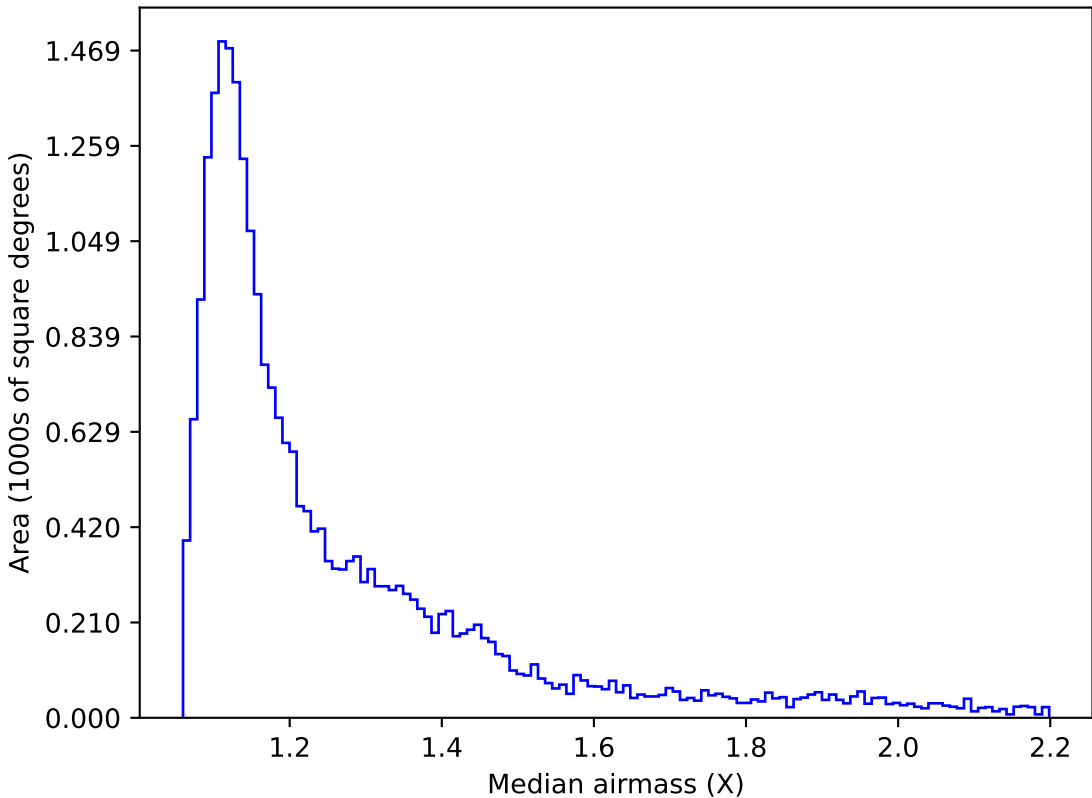
too_elab_r256_d3_ugrizy_v3.4_10yrs Yr 1 z band: Median airmass
