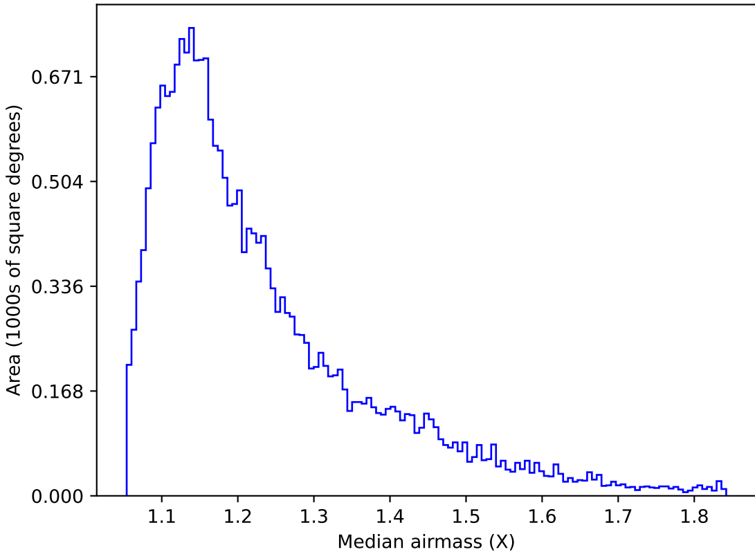
too_elab_r256_d3_ugrizy_v3.4_10yrs Yr 1 u band: Median airmass
