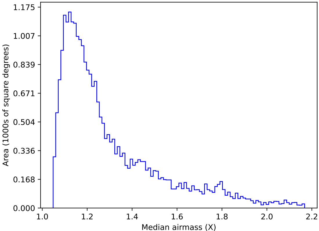
too_elab_r256_d3_ugrizy_v3.4_10yrs Yr 1 g band: Median airmass
