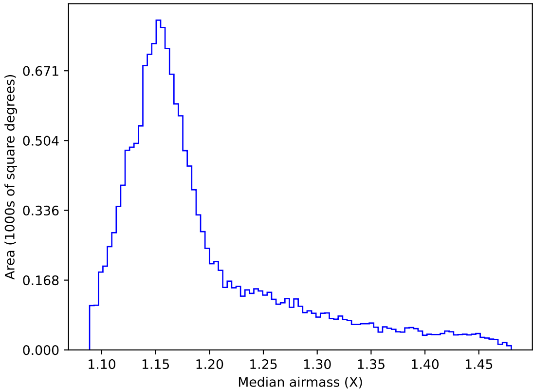
too_elab_r256_d3_ugrizy_v3.4_10yrs WFD z band: Median airmass
