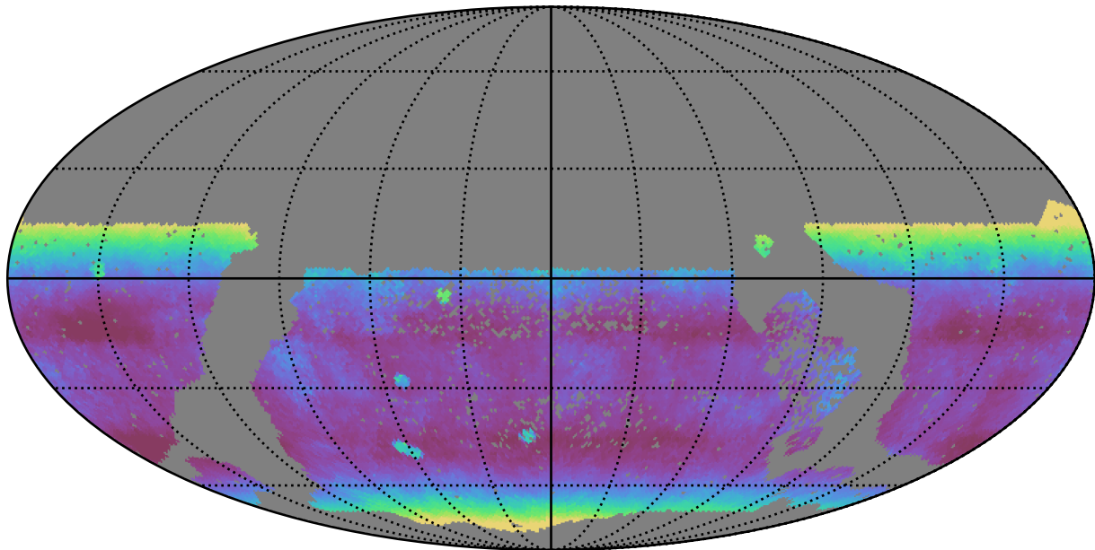
too_elab_r256_d3_ugrizy_v3.4_10yrs WFD y band: Median airmass
