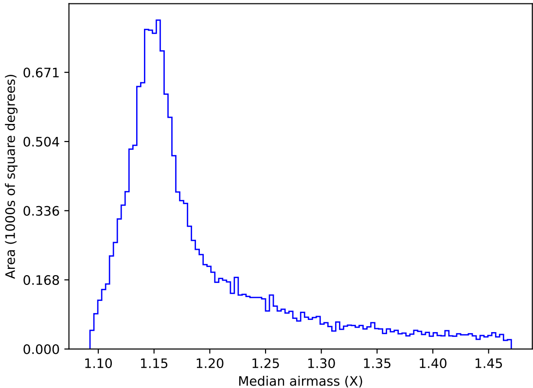
too_elab_r256_d3_ugrizy_v3.4_10yrs WFD y band: Median airmass
