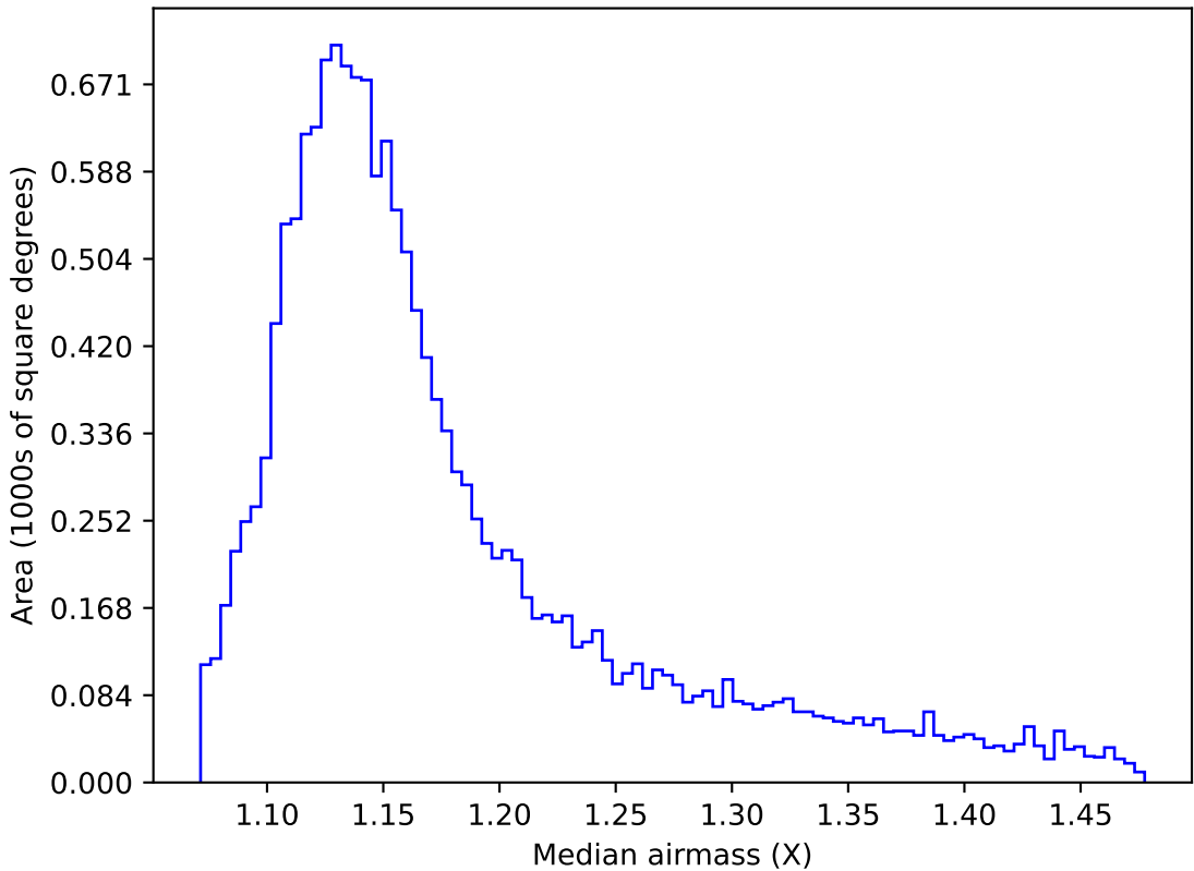
too_elab_r256_d3_ugrizy_v3.4_10yrs WFD u band: Median airmass
