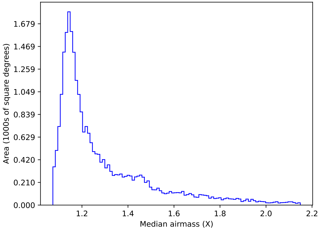
too_elab_r256_d3_ugrizy_v3.4_10yrs All sky g band: Median airmass
