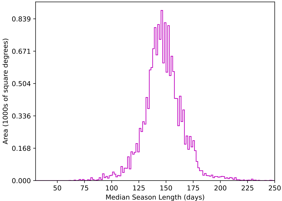
too_elab_r256_d3_ugrizy_v3.4_10yrs WFD z band: Median Season Length
