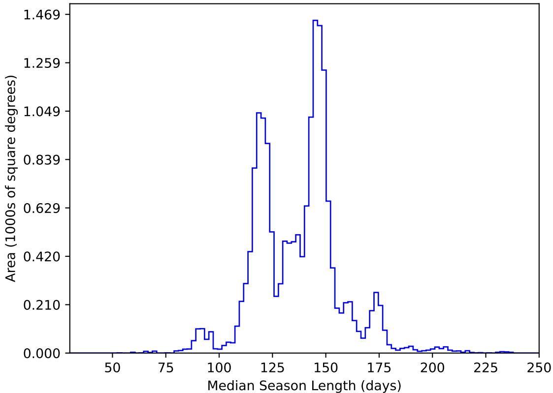
too_elab_r256_d3_ugrizy_v3.4_10yrs WFD y band: Median Season Length
