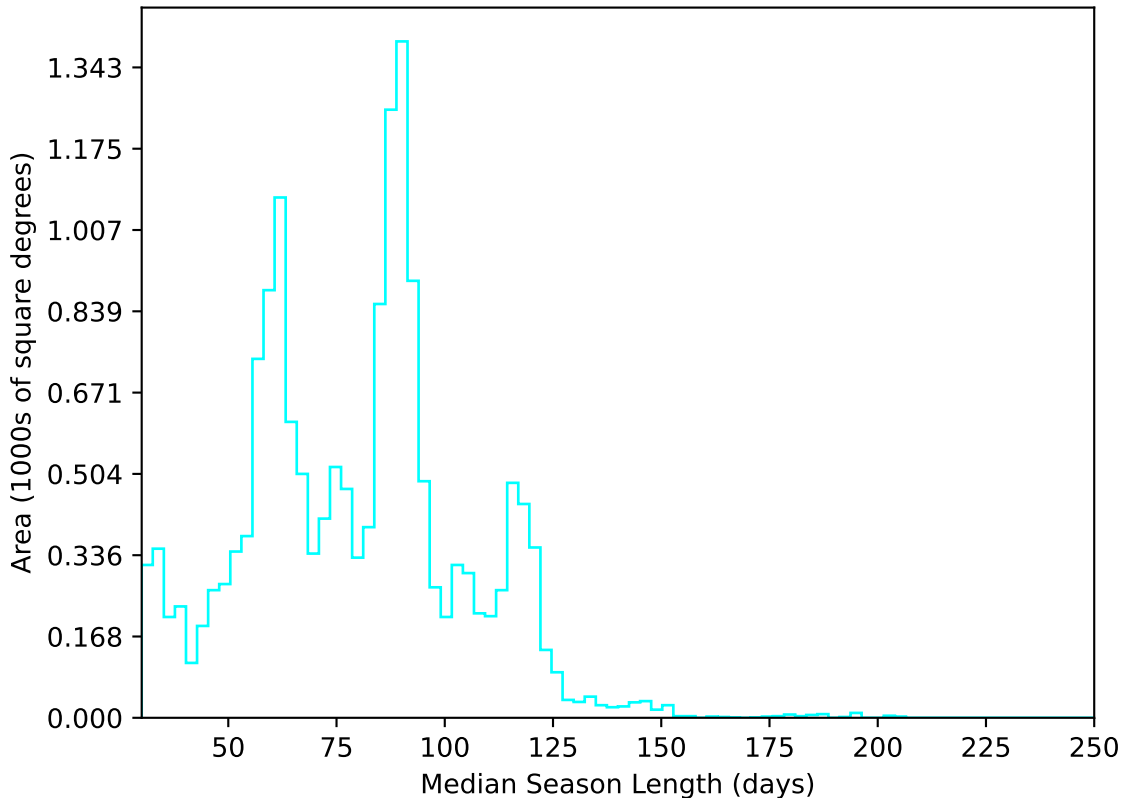
too_elab_r256_d3_ugrizy_v3.4_10yrs WFD u band: Median Season Length
