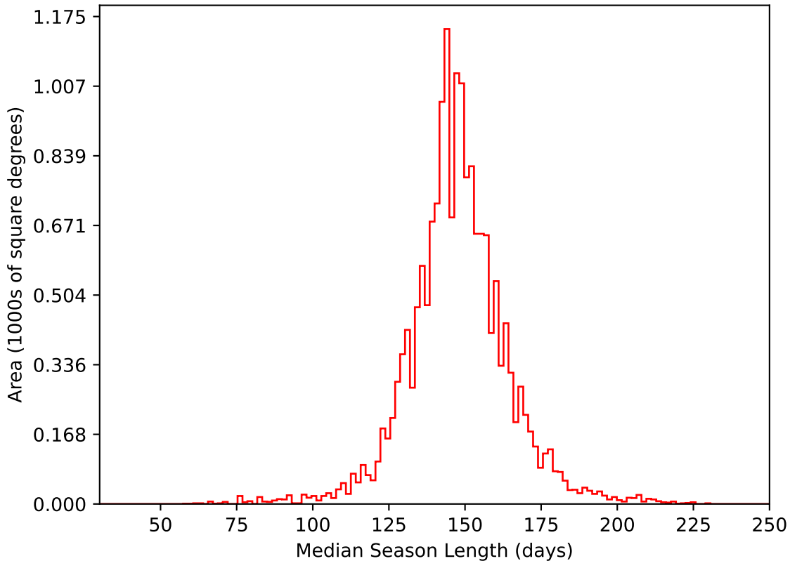
too_elab_r256_d3_ugrizy_v3.4_10yrs WFD i band: Median Season Length
