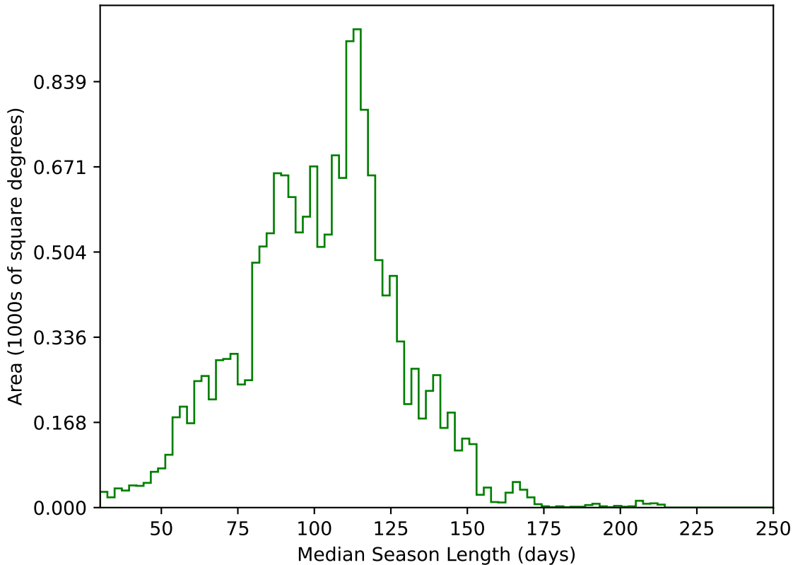
too_elab_r256_d3_ugrizy_v3.4_10yrs WFD g band: Median Season Length
