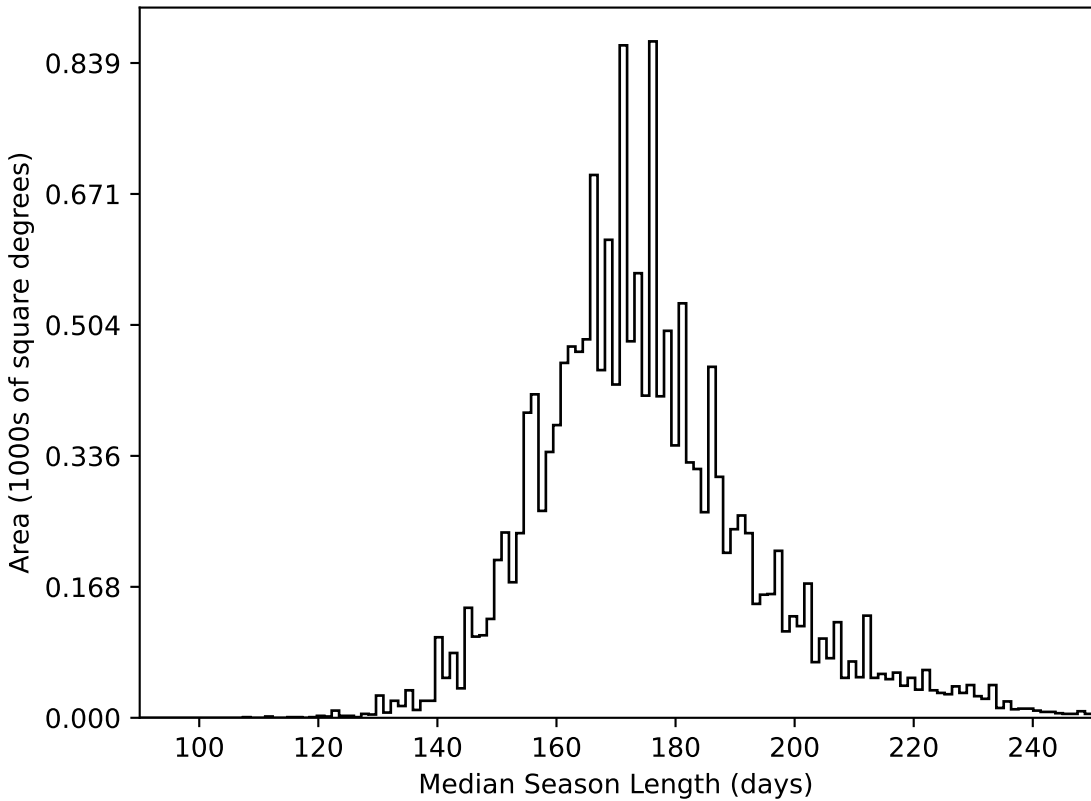
too_elab_r256_d3_ugrizy_v3.4_10yrs WFD all bands: Median Season Length
