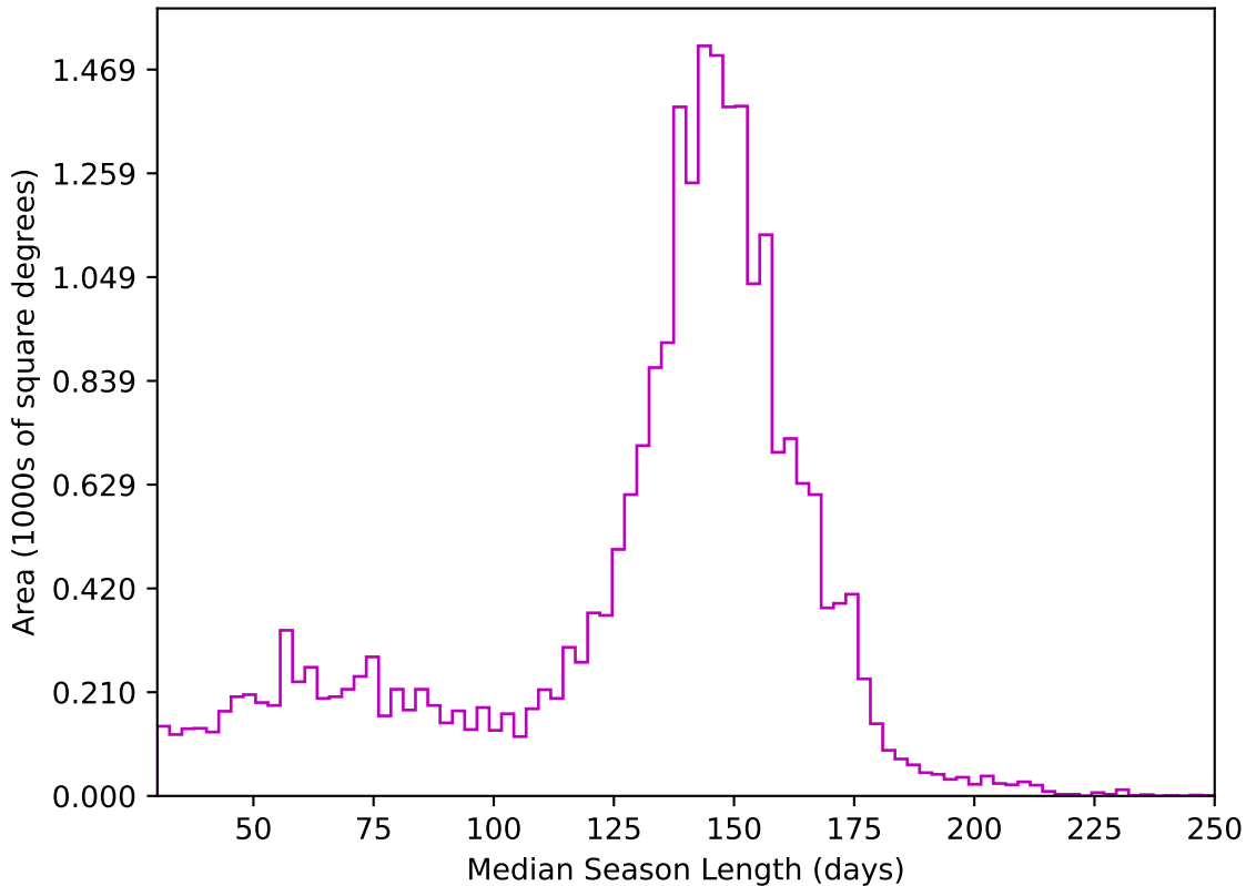
too_elab_r256_d3_ugrizy_v3.4_10yrs All sky z band: Median Season Length
