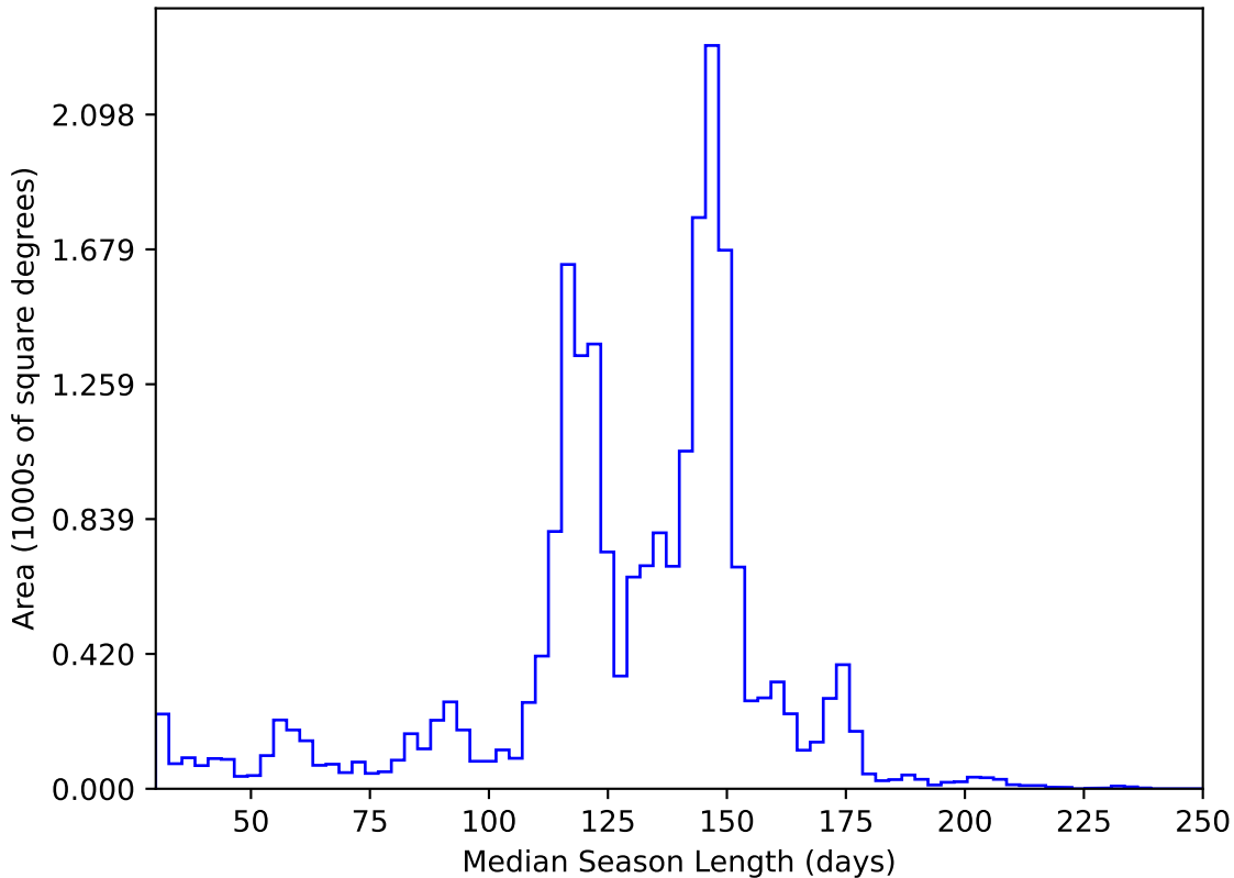
too_elab_r256_d3_ugrizy_v3.4_10yrs All sky y band: Median Season Length
