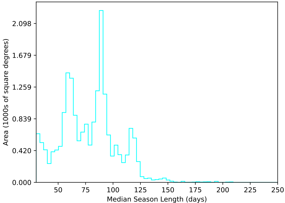
too_elab_r256_d3_ugrizy_v3.4_10yrs All sky u band: Median Season Length
