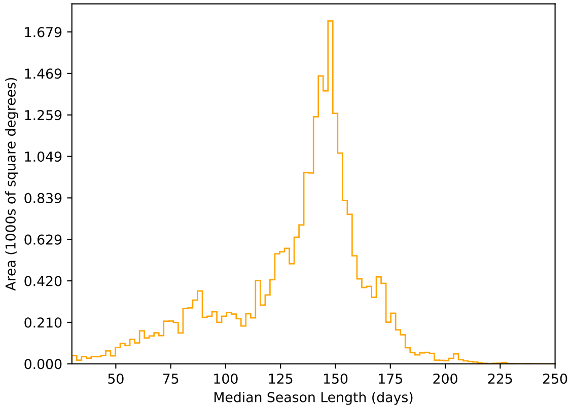
too_elab_r256_d3_ugrizy_v3.4_10yrs All sky r band: Median Season Length
