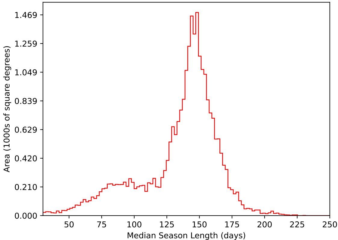
too_elab_r256_d3_ugrizy_v3.4_10yrs All sky i band: Median Season Length
