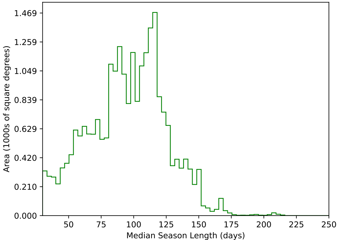
too_elab_r256_d3_ugrizy_v3.4_10yrs All sky g band: Median Season Length
