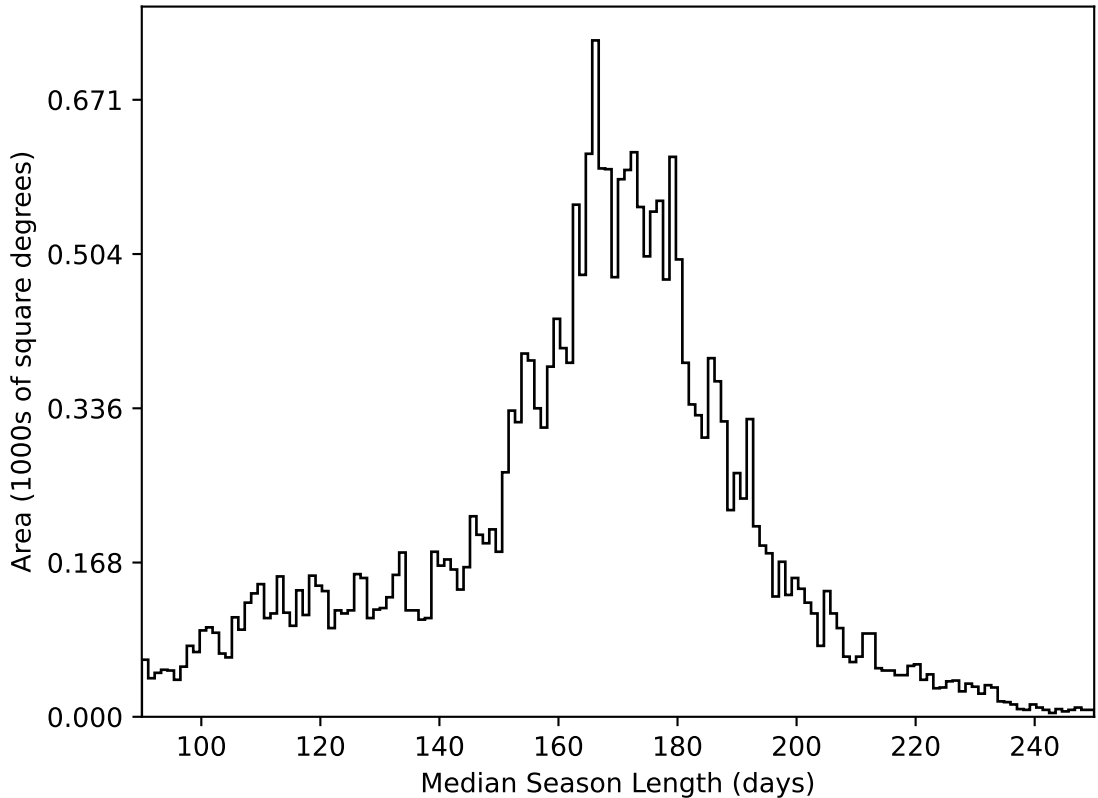
too_elab_r256_d3_ugrizy_v3.4_10yrs All sky all bands: Median Season Length
