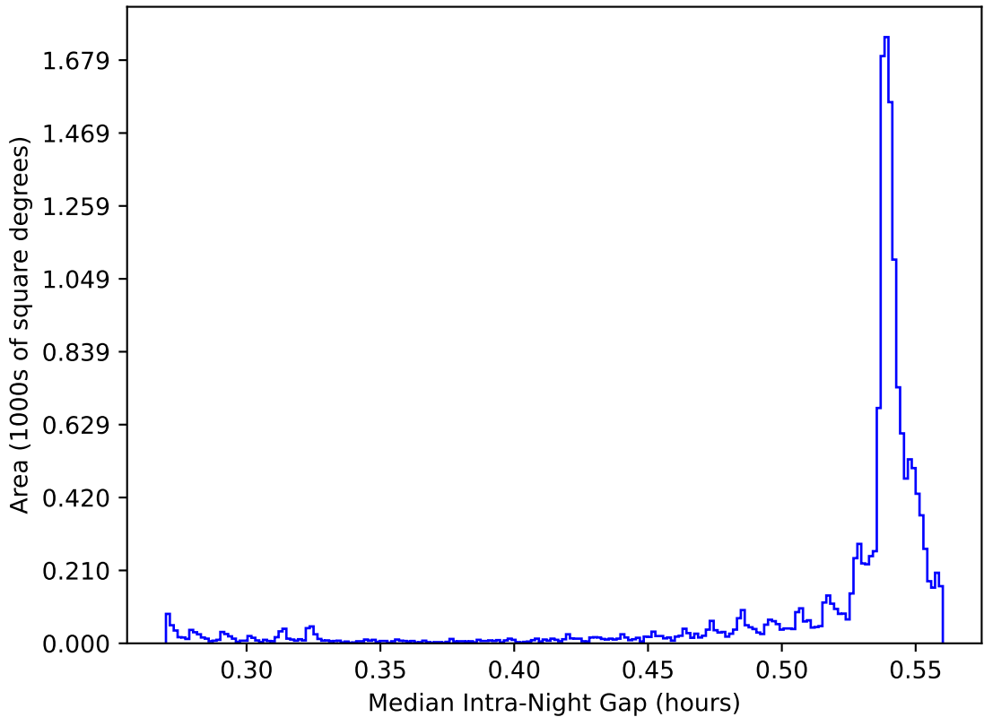
too_elab_r256_d3_ugrizy_v3.4_10yrs WFD: Median Intra-Night Gap
