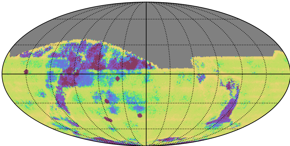
too_elab_r256_d3_ugrizy_v3.4_10yrs All sky: Median Intra-Night Gap
