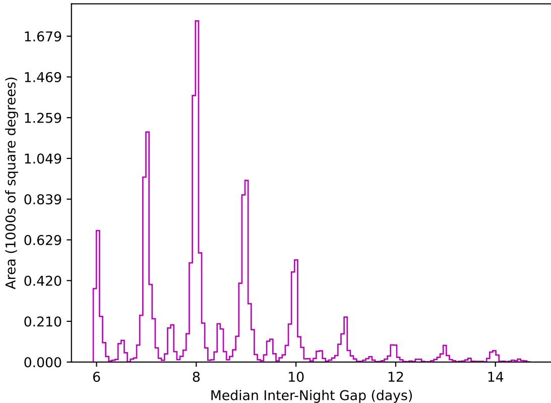
too_elab_r256_d3_ugrizy_v3.4_10yrs WFD z band: Median Inter-Night Gap
