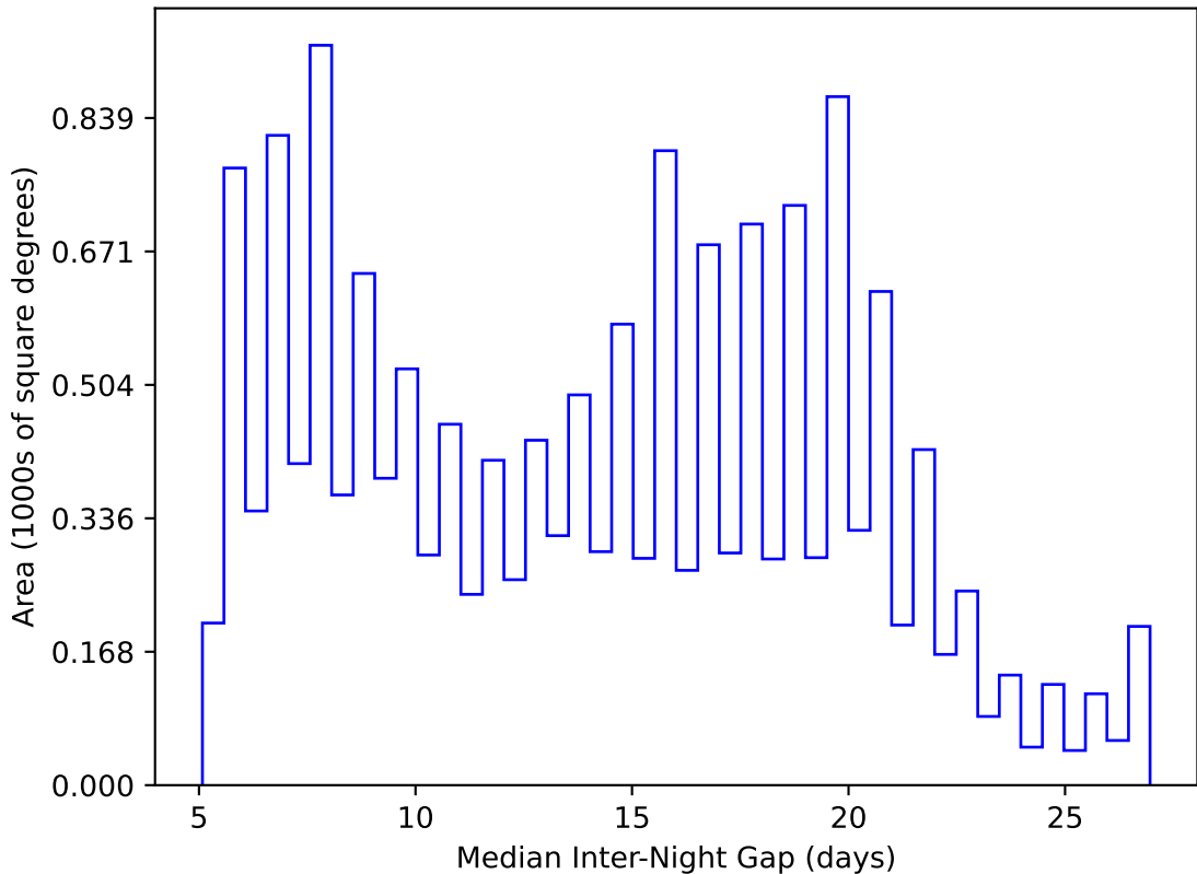
too_elab_r256_d3_ugrizy_v3.4_10yrs WFD y band: Median Inter-Night Gap
