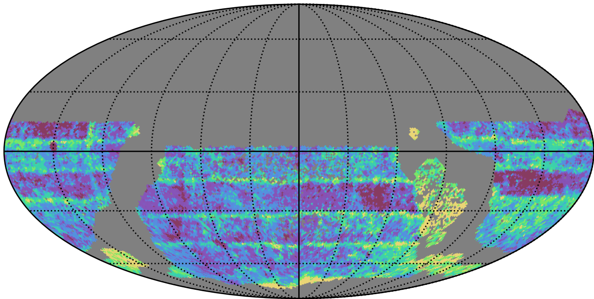
too_elab_r256_d3_ugrizy_v3.4_10yrs WFD i band: Median Inter-Night Gap
