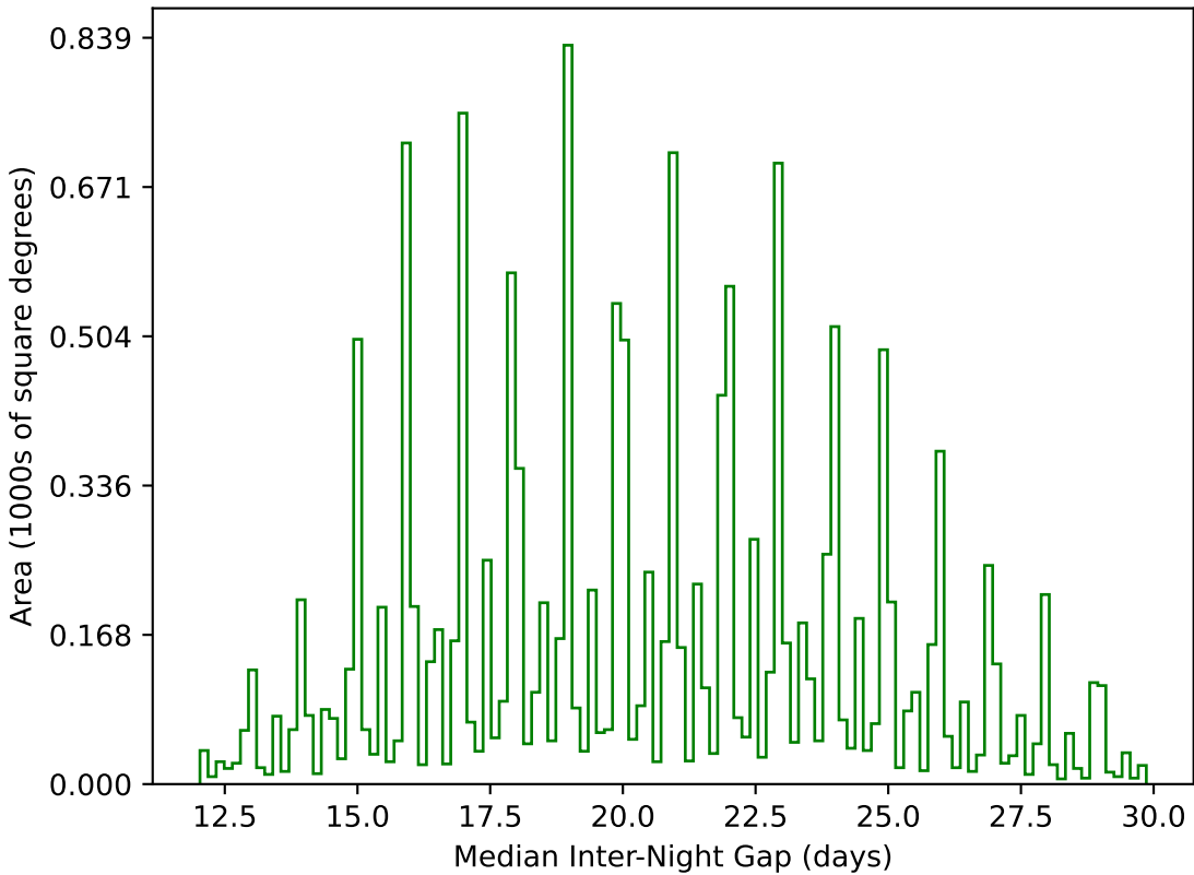
too_elab_r256_d3_ugrizy_v3.4_10yrs WFD g band: Median Inter-Night Gap
