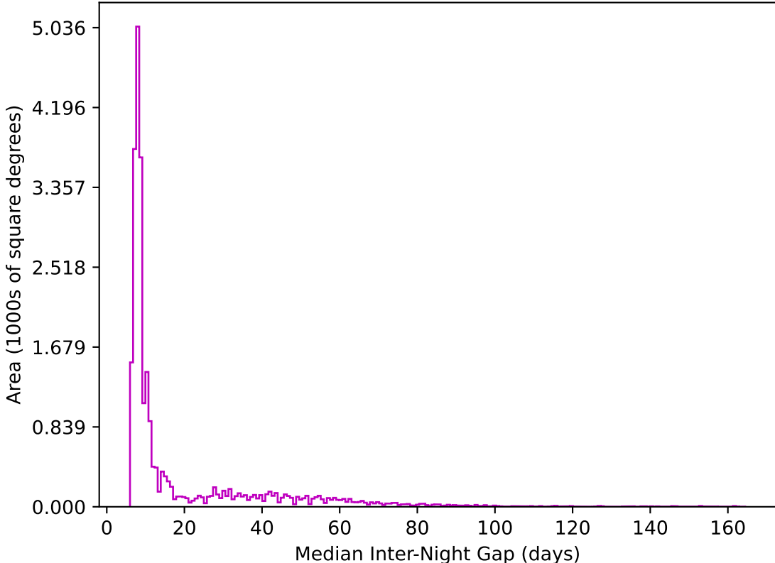
too_elab_r256_d3_ugrizy_v3.4_10yrs All sky z band: Median Inter-Night Gap
