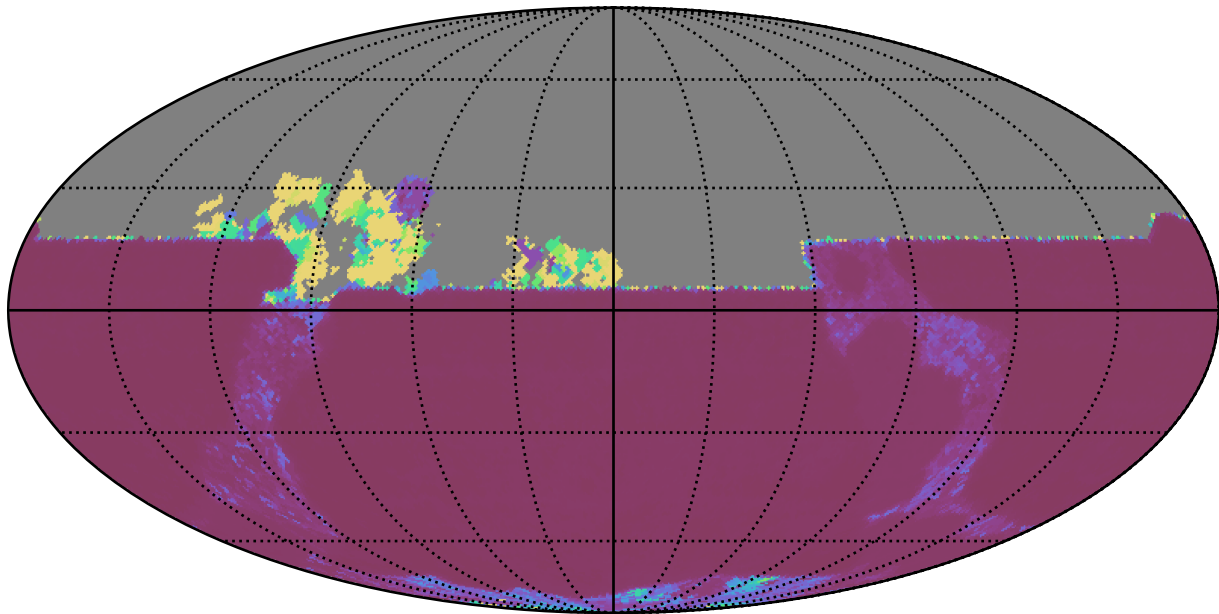
too_elab_r256_d3_ugrizy_v3.4_10yrs All sky y band: Median Inter-Night Gap
