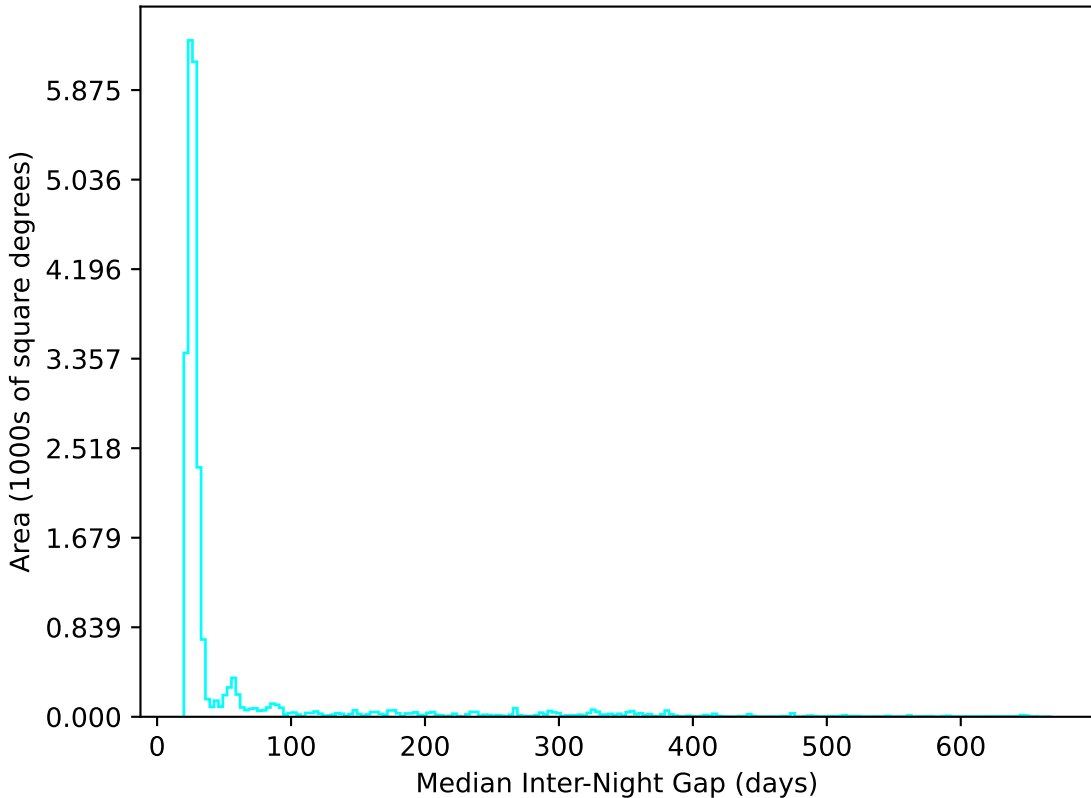
too_elab_r256_d3_ugrizy_v3.4_10yrs All sky u band: Median Inter-Night Gap
