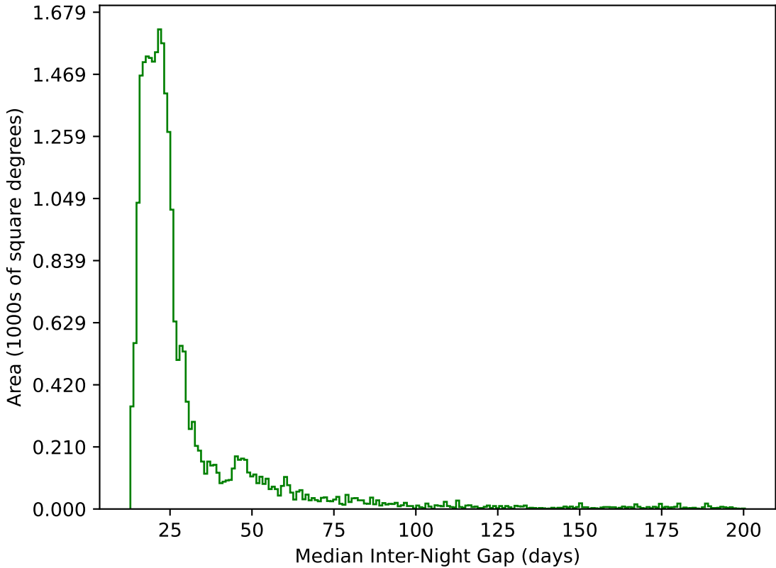
too_elab_r256_d3_ugrizy_v3.4_10yrs All sky g band: Median Inter-Night Gap
