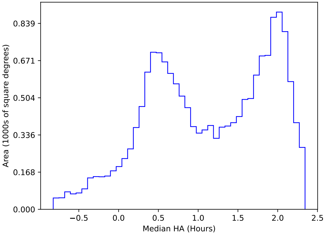
too_elab_r256_d3_ugrizy_v3.4_10yrs WFD z band: Median HA
